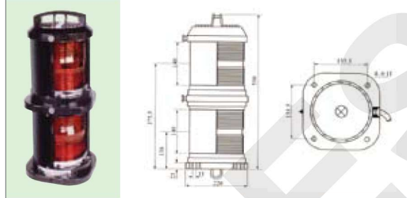
CXH2-10P - full plastic double - deck port light
