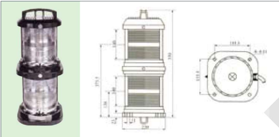
CXH3-10P - full plastic double - deck masthead light
